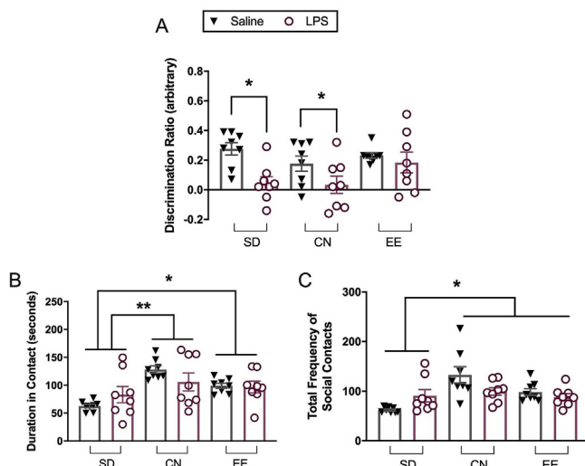
Fig. 2. Effects of maternal immune activation (MIA) on female offspring behavior. (A) MIA decreased spatial discrimination ability in an object-in-place task and environmental enrichment rescued this effect. Both (B) duration in social contact and (C) total frequency of social contacts were elevated by six weeks of postpubertal housing in environmental complexity. Saline = solid black triangles, LPS = open maroon circles. Data represent mean expression ( \pm SEM); * p < 0.05 , ** p < 0.01 , n = 8 litters for each group.
